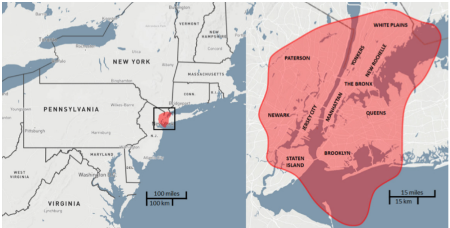
Figure 3: Equivalent area of destruction for a Tunguska-sized asteroid over New York City. (OSTP)
