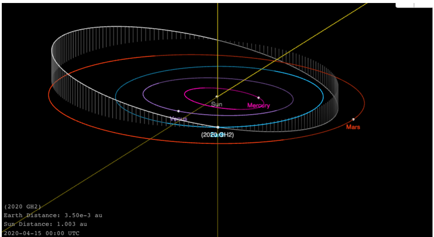
2020 GH2 crosses earth's orbit on April 15, 2020. (NASA JPL)
