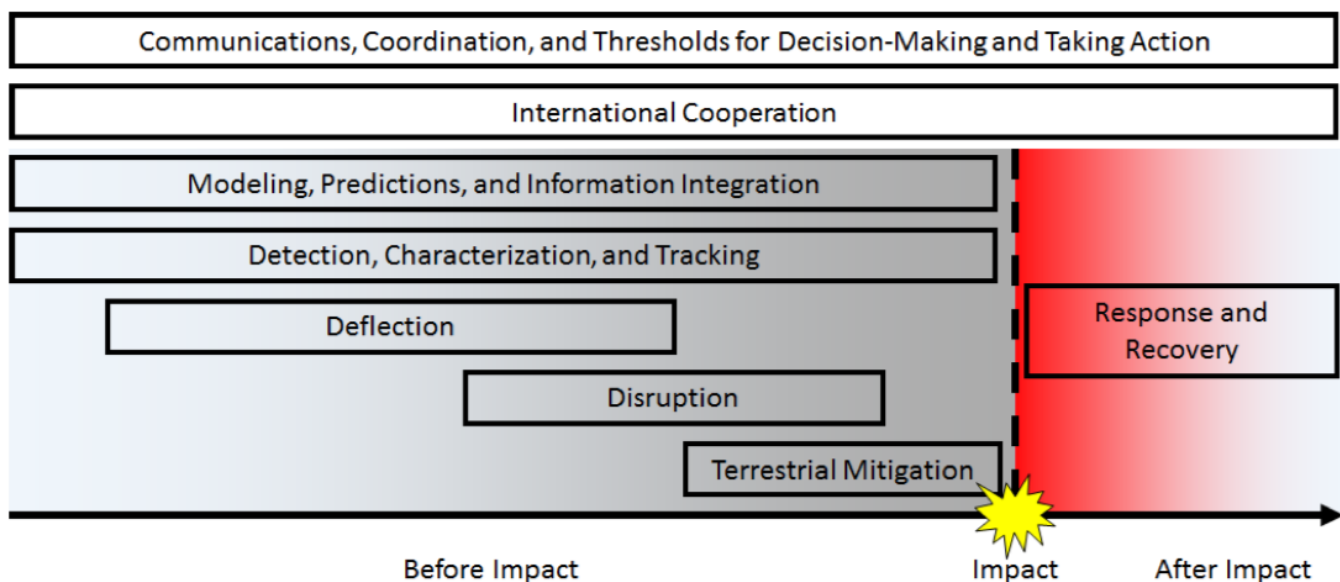
Figure 5: Illustrative timeline of the potential phases of operations in a NEO threat scenario. (OSTP)
